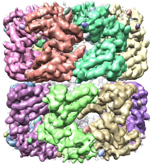
Regions grouped based on fitted models.
