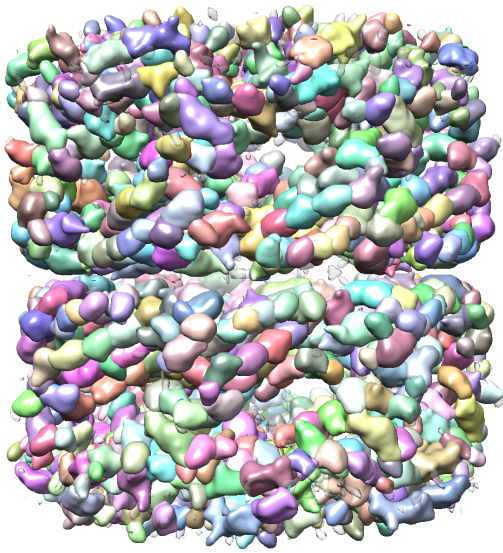
All watershed regions in the map
